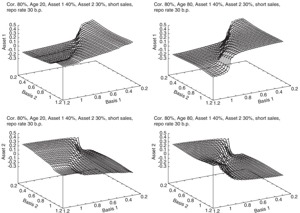
Fig. 4. Optimal portfolio choice with short sales allowed, \pi_1 = 0.4 , \pi_2 = 0.3 , \rho = 0.8 , and shorting costs of 30 basis points. The investor enters the age t trading period with 40% (30%) of his wealth invested in stock 1 (2). In the left panels the investor is age 20, while in the right panels the investor is age 80. The top (bottom) panels plot the optimal allocation of stock 1 (2) as a function of the basis-price ratios of the two stocks. The investor can sell short subject to a shorting cost of 30 basis points.
